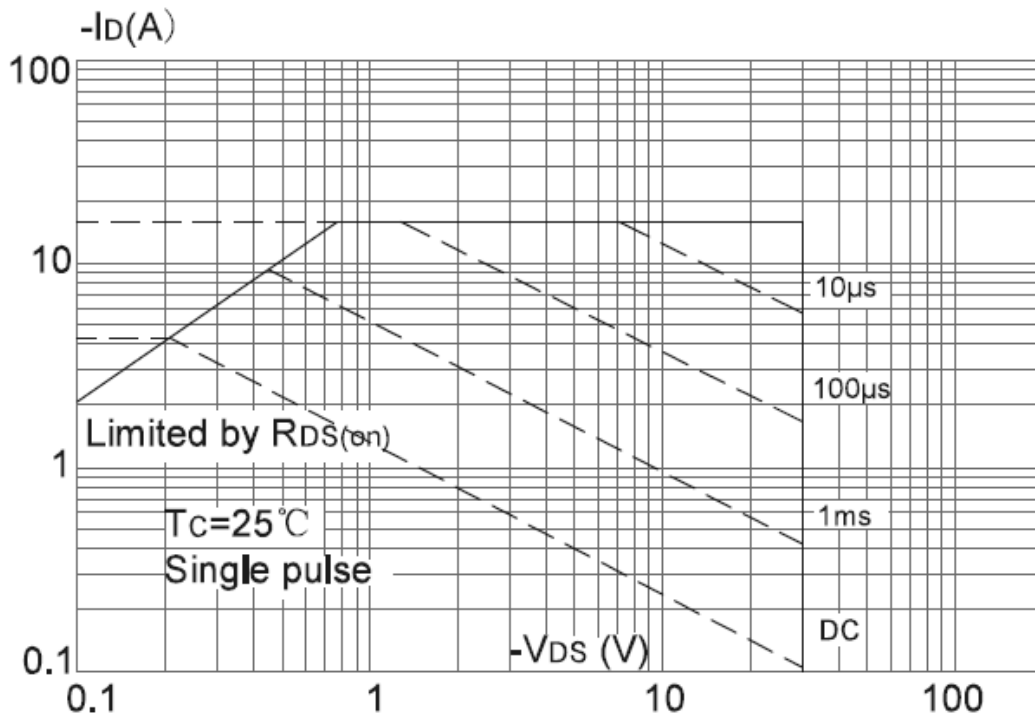
Fig.10 Maximum Safe Operating Area
