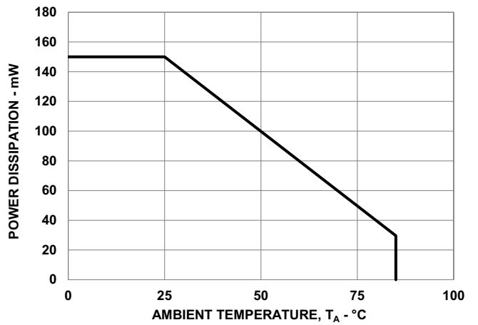
Figure 11: Power Dissipation vs. Ambient Temperature
