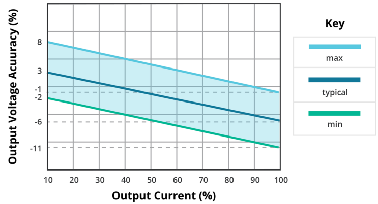
OUTPUT REGULATION CURVE VQA3S-S5-D18-S (-Vo)
