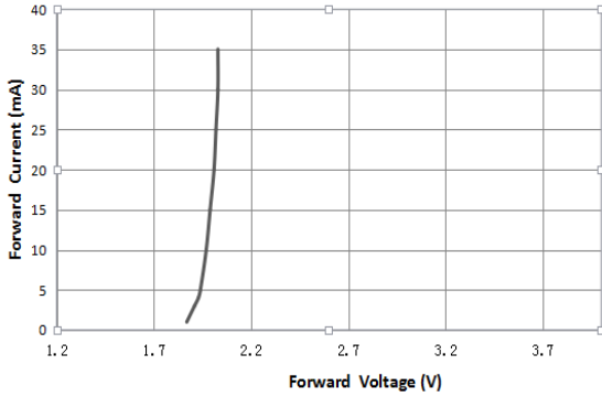
Forward Current VS. Forward Voltag (Ta=25°C)
