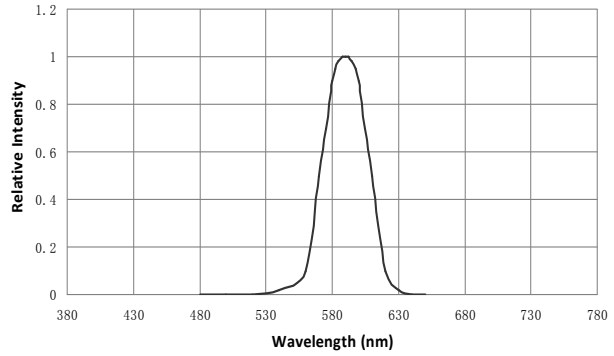
Spectrum Distribution (Ta=25°C)
