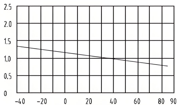
LUMINOUS INTENSITY VS AMBIENT TEMPERATURE 亮度与环境温度关系曲线图
