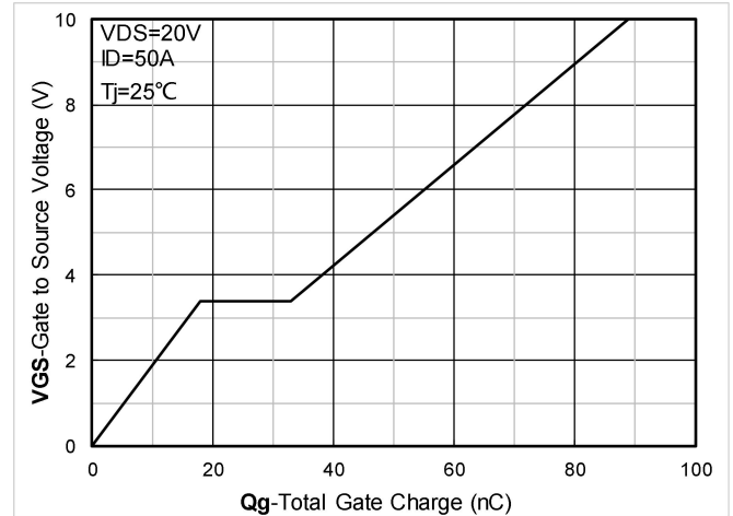
Figure 4. Gate Charge
