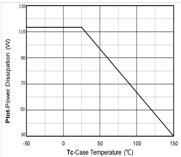
Figure 11. Power dissipation
