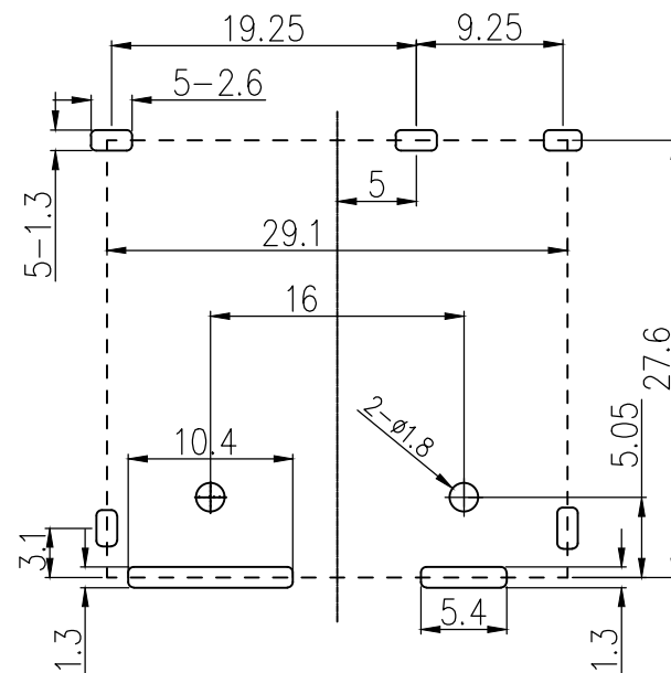
PCB Layout
