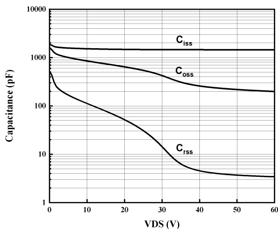
Fig5. Typical Capacitance
