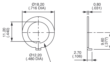
LOCKING RING
