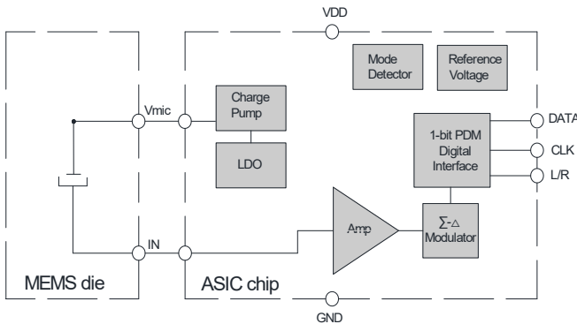
Fig. 1 Microphone block diagram
