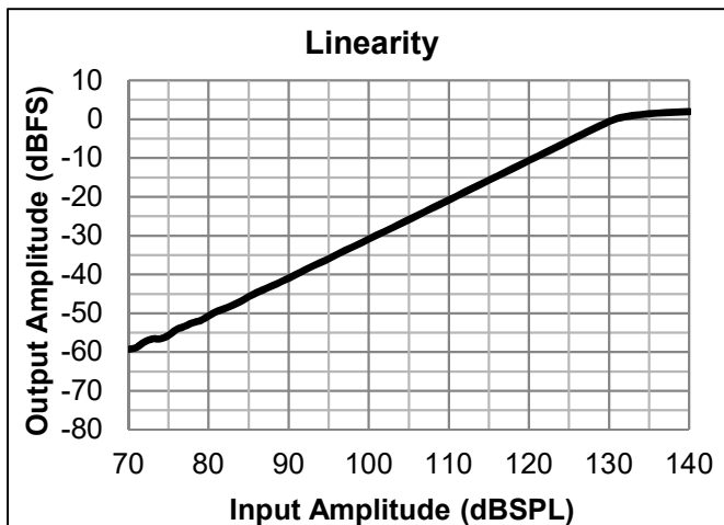
Fig. 8 Linearity
