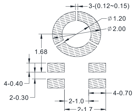
Example Solder Stencil Pattern
