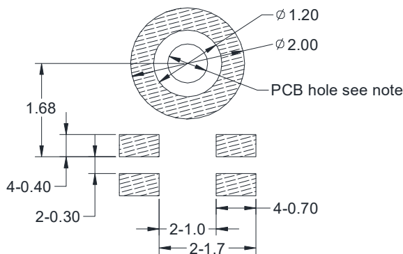
Example Land Pattern
