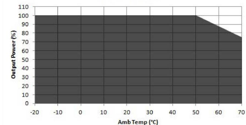
Figure 1. Derating Curve
