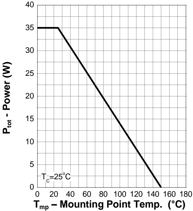
Power Capability
