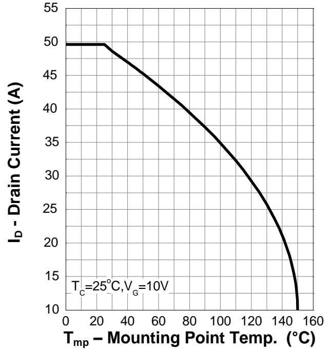
Current Capability
