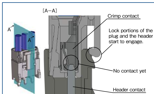
Lock structure
