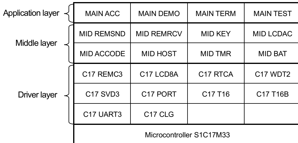
Functional Blocks
