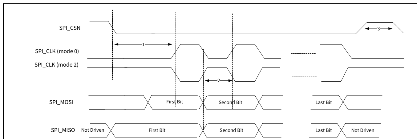
Figure 12 SPI timing, mode 0 and 2
