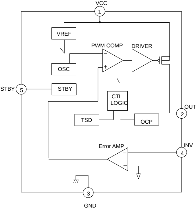
Figure 2. Block Diagram
