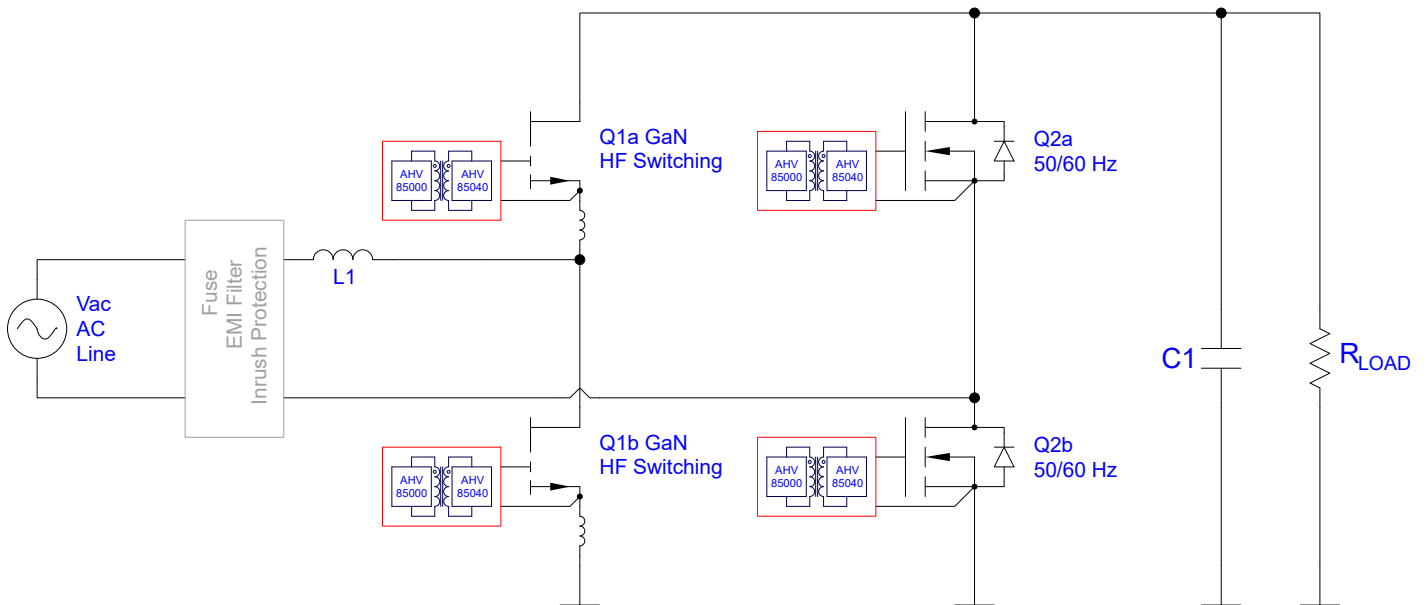
Figure 12: Totem Pole PFC with AHV85000 + AHV85040 Chipset as High-Side and Low-Side Drivers
