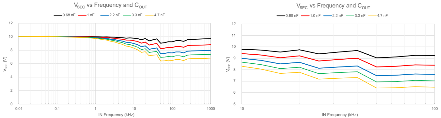
Figure 8: Secondary-Side Voltage, V_{SEC} , vs. Frequency and C_{OUT} Conditions: V_{DRV} = 12\text{ V} , C_{SEC} = 100\text{ nF} , X_{FMR} = \text{SM91234L} , T_A = 25^\circ\text{C}
