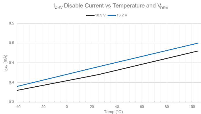
I_{DRV} Disable Current vs. Temperature and V_{DRV}
