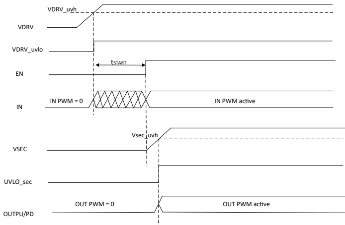
Figure 4: Startup Mechanism
