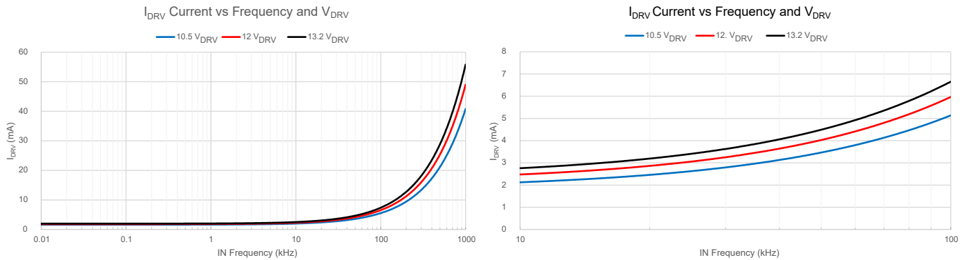
Input Current vs. Frequency and V_{DRV}
