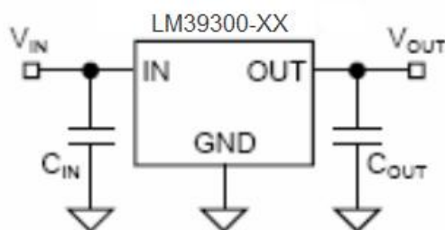
Fig 1. Capacitor Requirements
