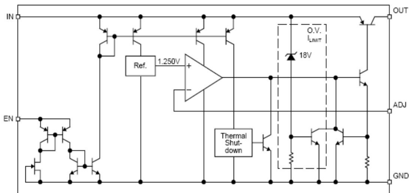
LM39302 Adjustable
