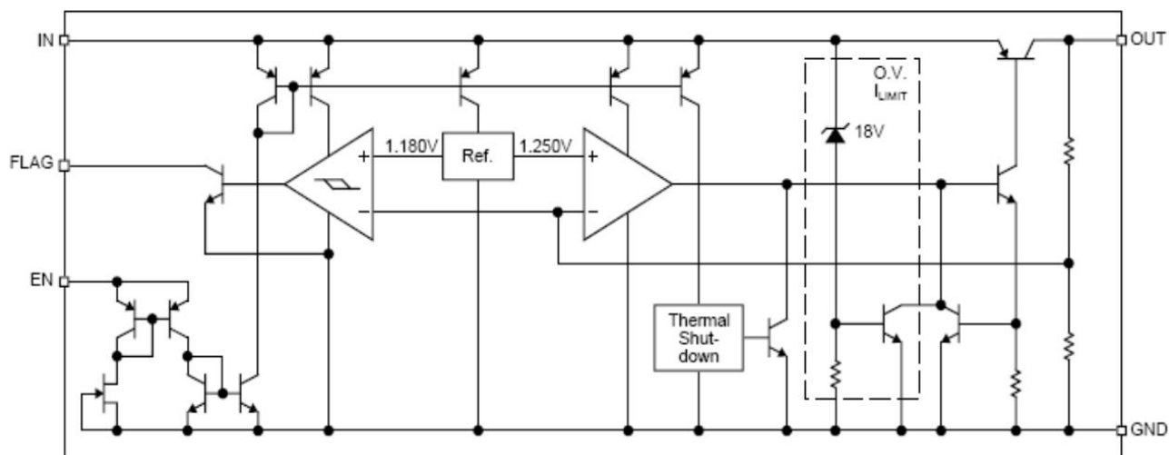
LM39301 Fixed with flag and enable
