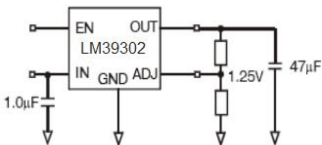
LM39302
