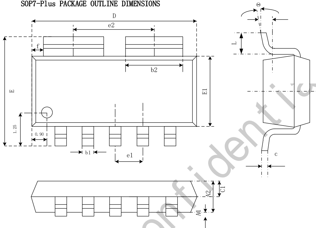
SOP7-P1us PACKAGE OUTLINE DIMENSIONS
