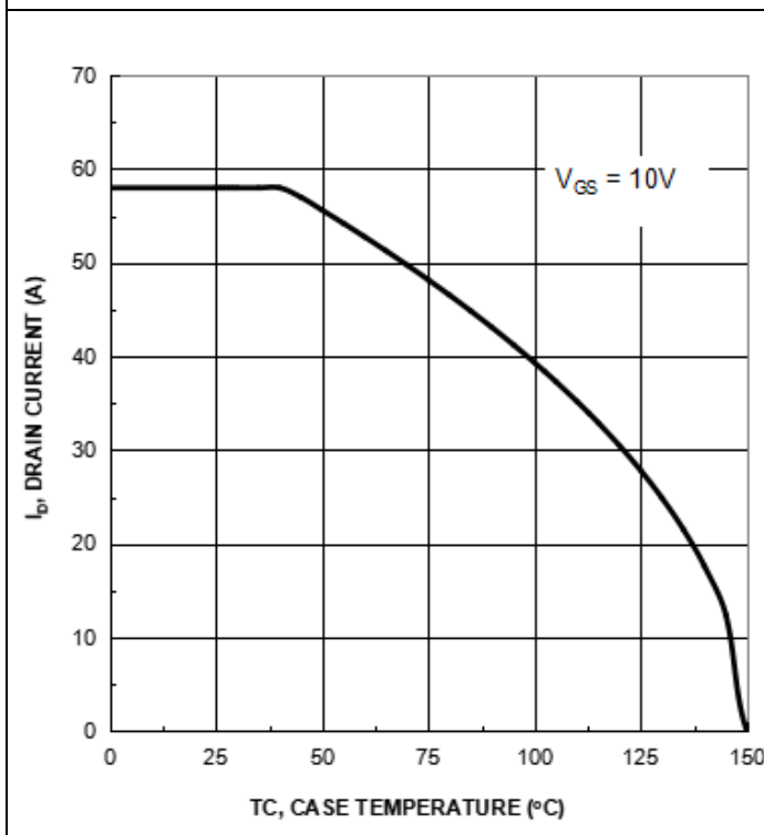
Fig 7, Current Rating
