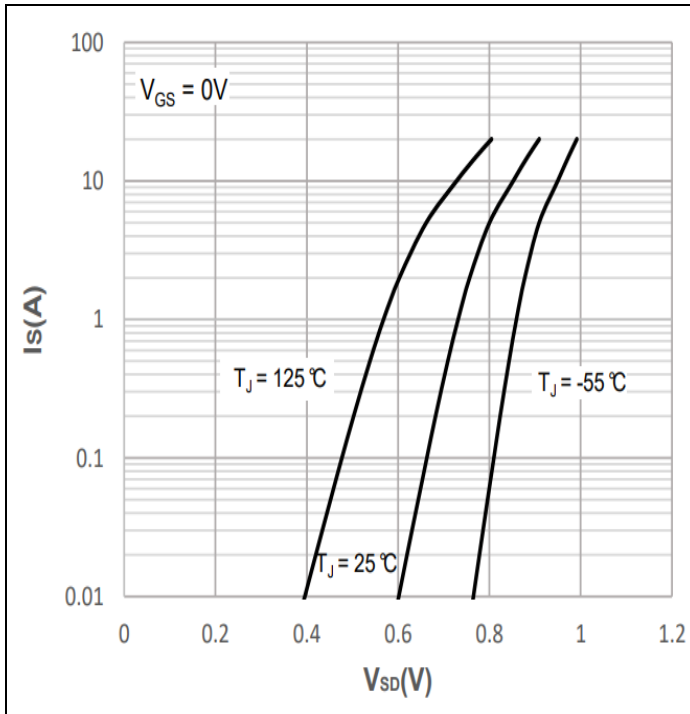
Fig 5, Body Diode Characteristics
