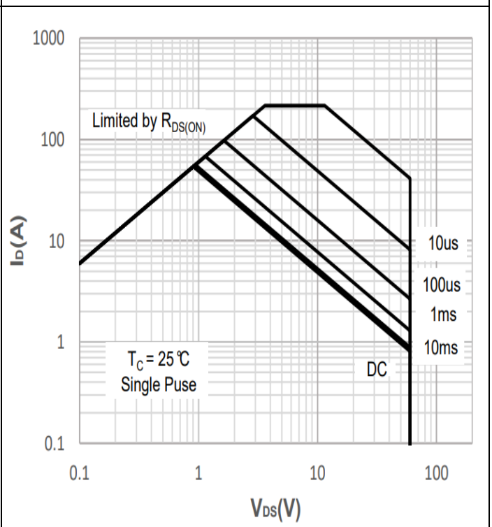
Fig 8, Maximum Safe Operating Area
