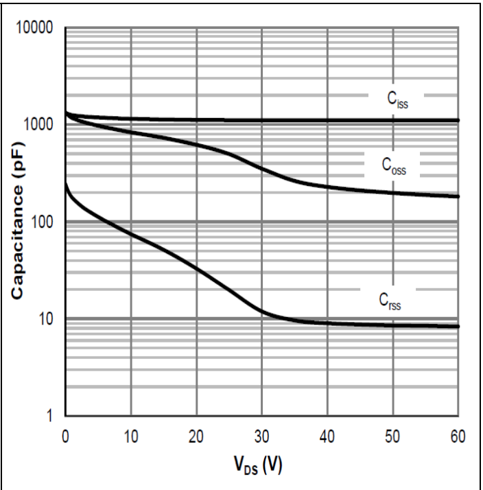
Fig 6, Typical Capacitance vs. Drain-to-Source Voltage
