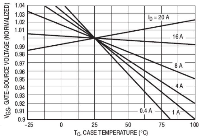
Figure 7. Gate-Source Voltage versus Case Temperature
