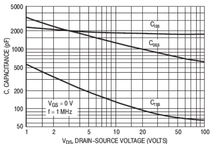
Figure 5. Capacitance versus Drain Voltage
