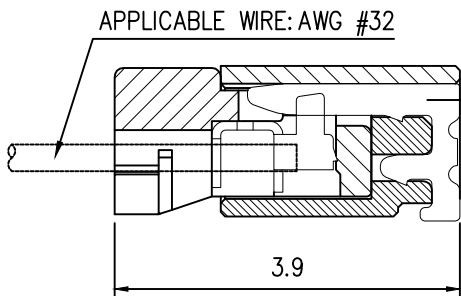
MATED CONDITION
