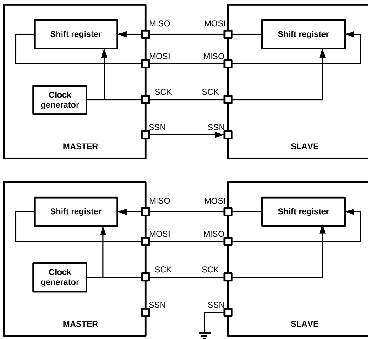
图 23-7 SPI Master/SPI Slave 互连
