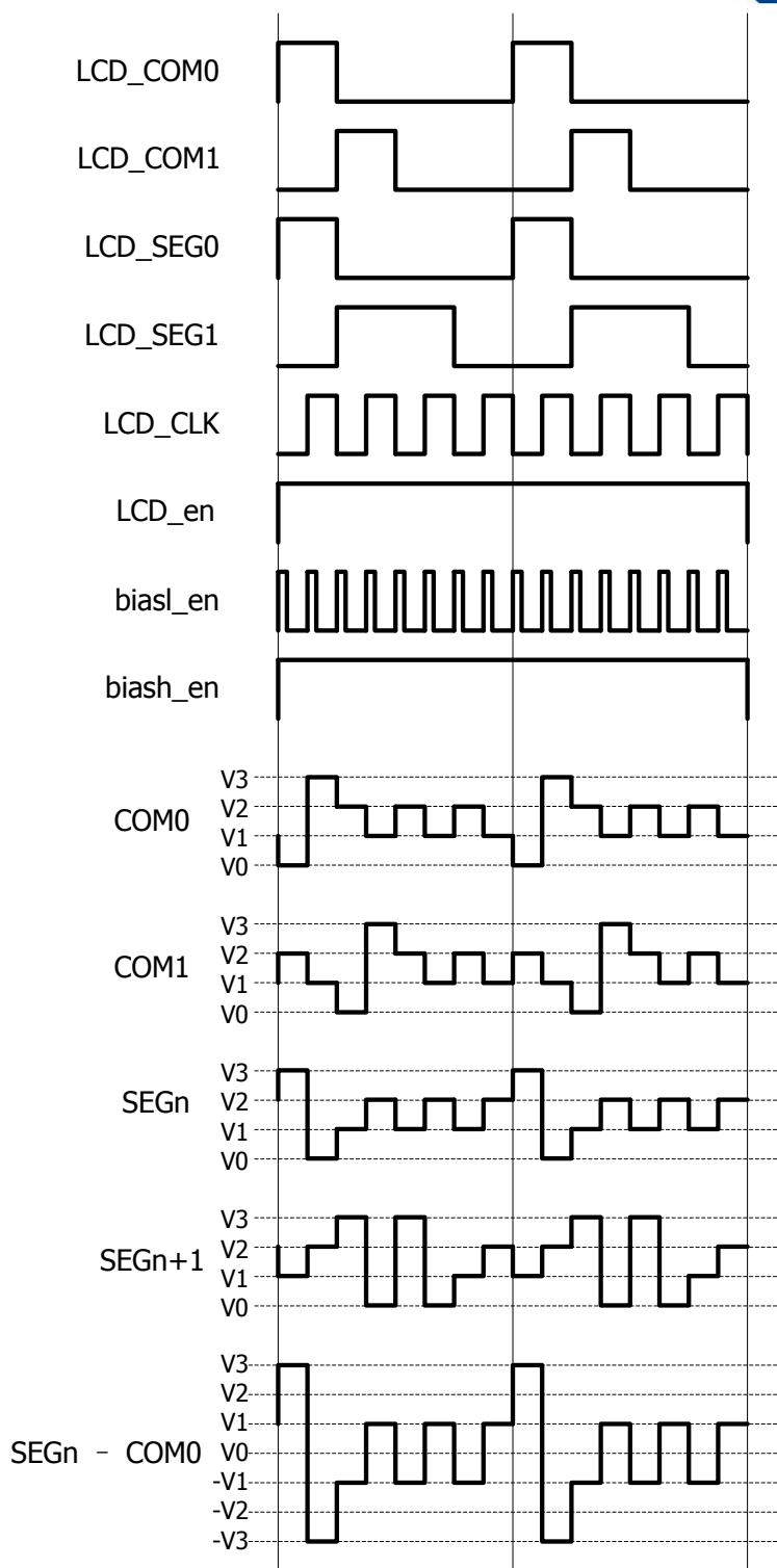
图 32-2LCD 驱动波形(1/4 duty, 1/3 bias, type A)
