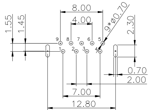
RECOMMENDER P.C.B.LAYOUT TOP VIEW (COMPONENT SIDE TOLERANCE±0.05)
