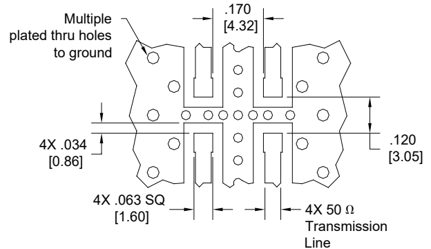
Dimensions are in Inches [Millimeters] 1P520* Mounting Footprint
