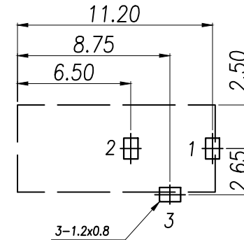
PCB.WELDING DRAWING (TOLERANCE:±0.05)
