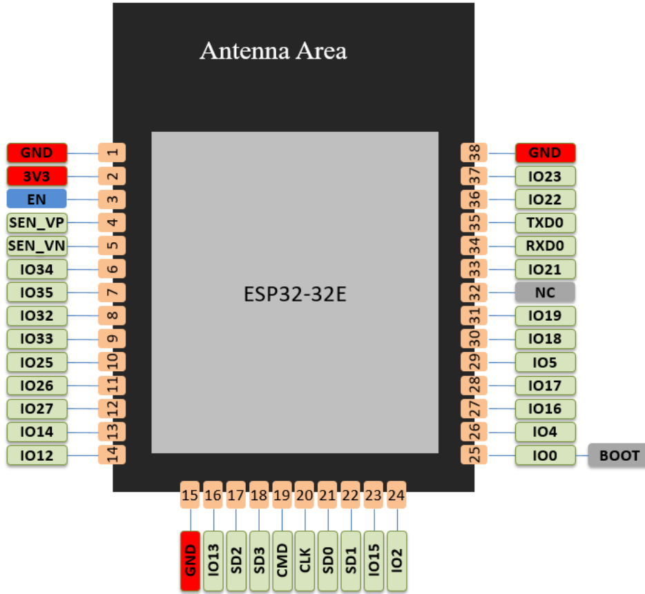
Fig.2.1 ESP32-32E Pins Definition
