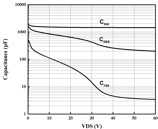
Fig5. Typical Capacitance
