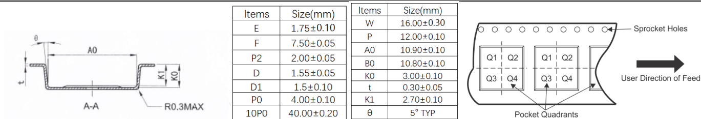
Note: The Pin 1of the chip is in the quadrant Q1 Figure 26.16-Lead Wide Body SOIC [WB SOIC-16] Reel Information
