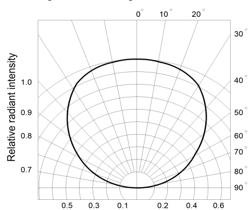
Fig.6 Radiation diagram
