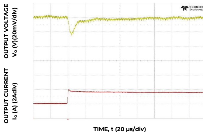
Figure 10. Transient Response to Dynamic Load Change from 50% to 100% at 12Vin, C_o=8 \times 47 \mu\text{F} , C_{Tune}=4.7 \text{nF} , R_{Tune}=300
