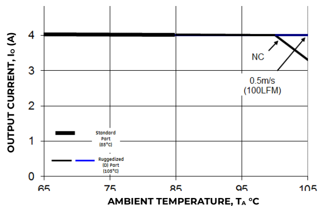
Figure 32. Derating Output Current verses Ambient Temperature
