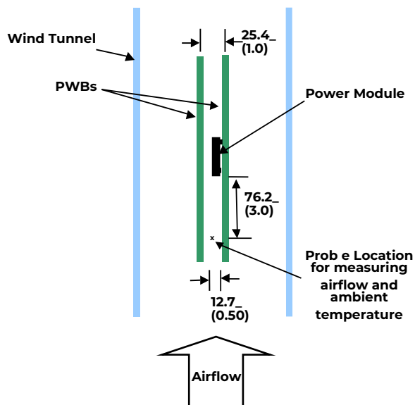
Figure 48. Thermal Test Set-up.
