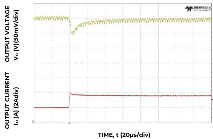
Figure 22. Transient Response to Dynamic Load Change from 50% to 100% at 12Vin, C_{out}=3 \times 47\mu\text{F} , C_{Tune}=1.5\text{nF} , R_{Tune}=300
