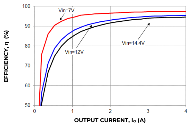
Figure 31. Converter Efficiency verses output current
