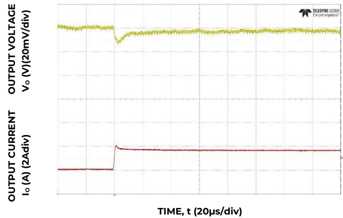
Figure 4. Transient Response to Dynamic Load Change from 50% to 100% at 12V in , C_{out}=4 \times 47\mu\text{F} + 2 \times 330\mu\text{F} , C_{Tune}=15\text{nF} , R_{Tune}=300
