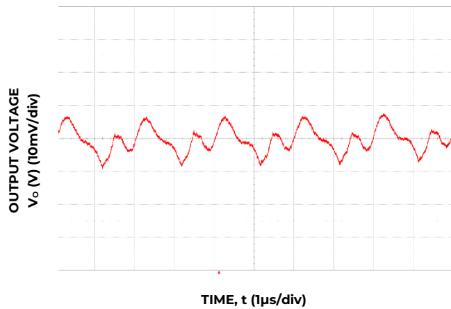
Figure 15. Typical output ripple ( C_o=3 \times 22\mu\text{F} ceramic, V_{IN} = 12\text{V} , I_o = I_{o,max} ).
