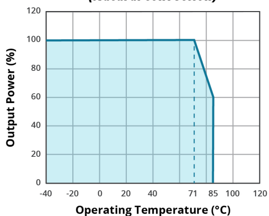
TEMPERATURE DERATING CURVE -3.3, -5, -6.5V output (Natural convection)
