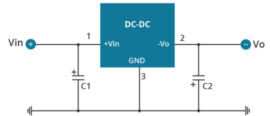
Figure 1 negative output
