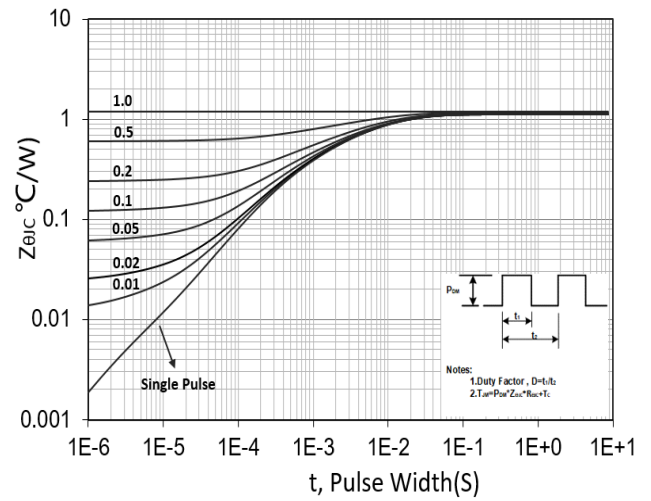
Figure 14. Transient Thermal Response Curve (TO-252)
