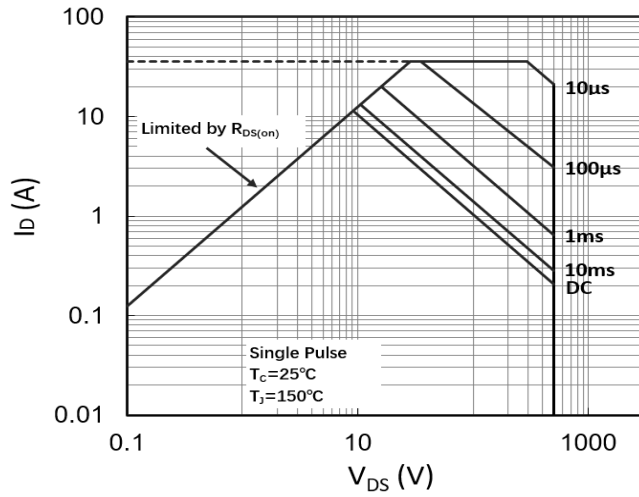
Figure13. Maximum Safe Operating Area (TO-252)
