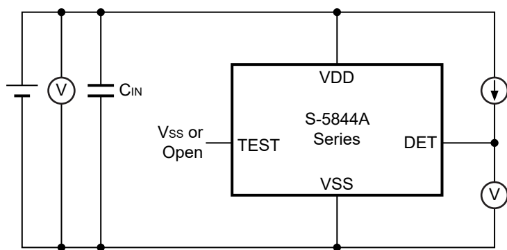
Figure 8 Test Circuit 3
