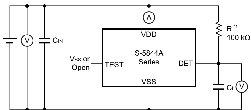
Figure 6 Test Circuit 1
