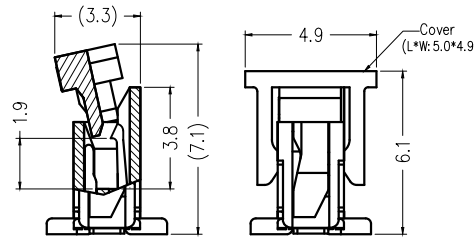
SECTION A-A WITH COVER
