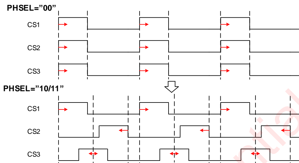
Figure 22 Three-Phase Mode
