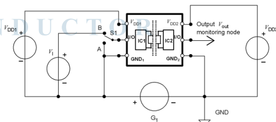
Figure 17. Common-mode transient immunity (CMTI) measurement
