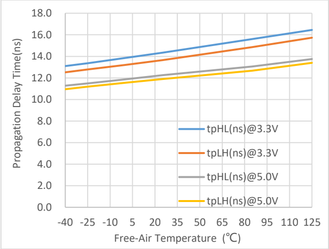
Figure 12. \pi 12\text{xM}6\text{x} Propagation Delay Time vs. Free-Air Temperature
