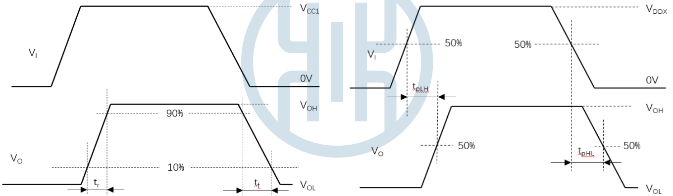
Figure 13. Transition time waveform measurement
