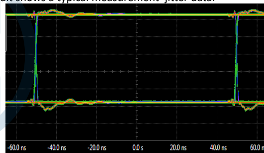
Figure 16. \pi 120\text{Mxx}/\pi 121\text{Mxx}/\pi 122\text{Mxx} Eye Diagram
