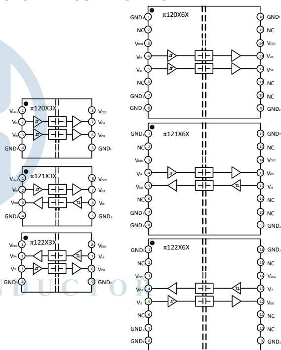
Figure 1. \pi 120xxx/\pi 121xxx/\pi 122xxx functional Block Diagram
