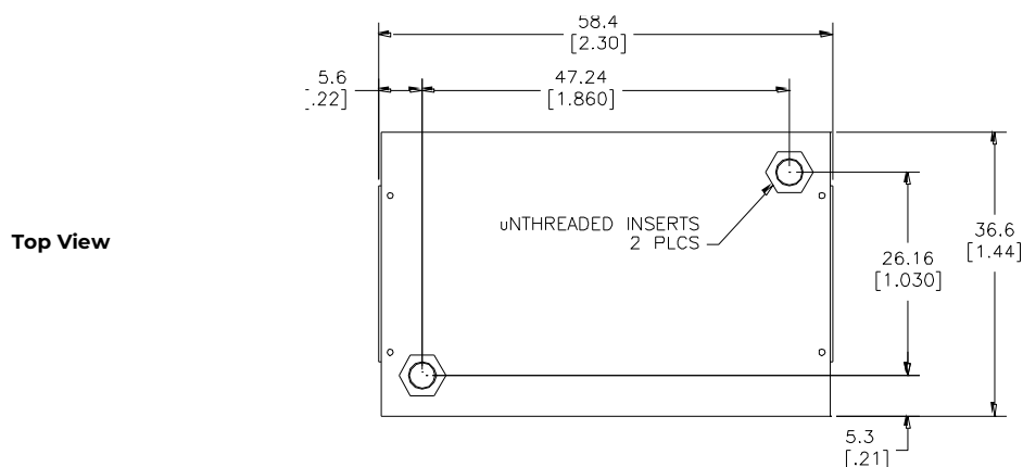
Mechanical Outline for EHHD_120W Through-Hole Module with 1/4th Brick Heat Plate
