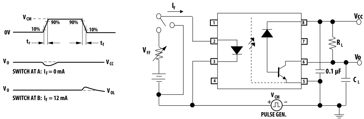
Figure 13: Test Circuit for Transient Immunity and Typical Waveforms
