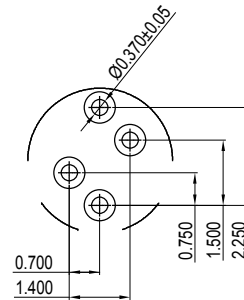
DETAIL W SCALE 8:1
