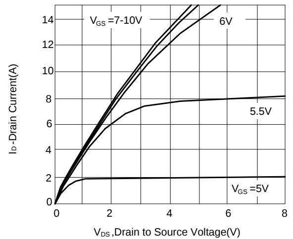
Figure 10: Output Characteristics
