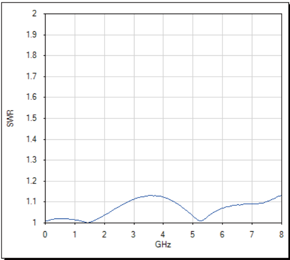
■ Insertion Loss
