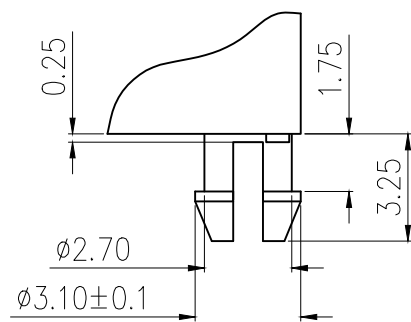
DETAIL "X" SCALE 2:1
