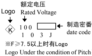
■图纸 Drawing
