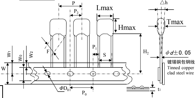
■图纸 Drawing
