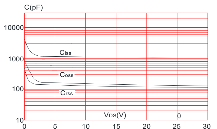
Figure 6: Capacitance Characteristics
