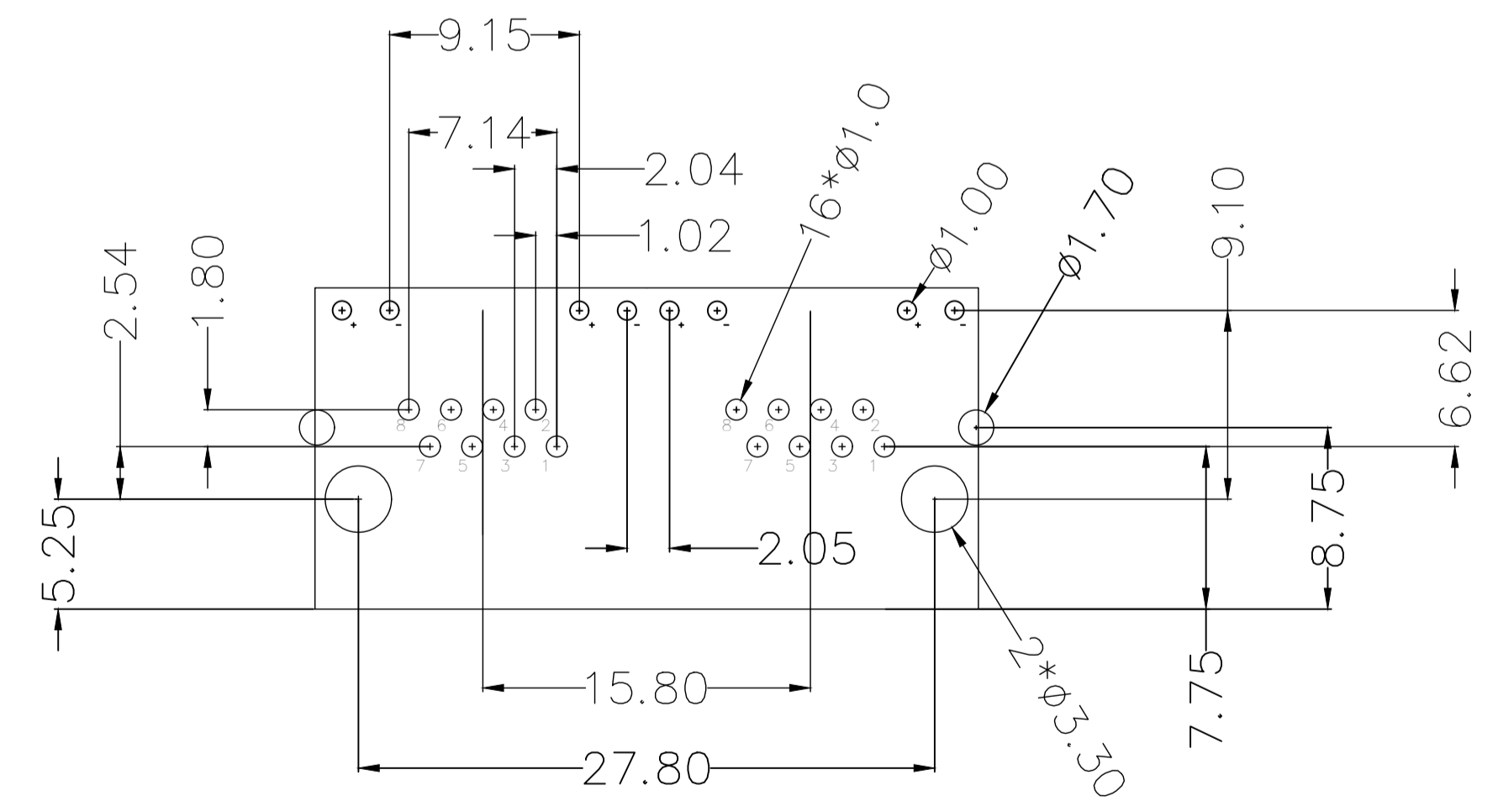
RECOMMENDED PCB LAYOUT TOP VIEW(TOL: ±0.05)
