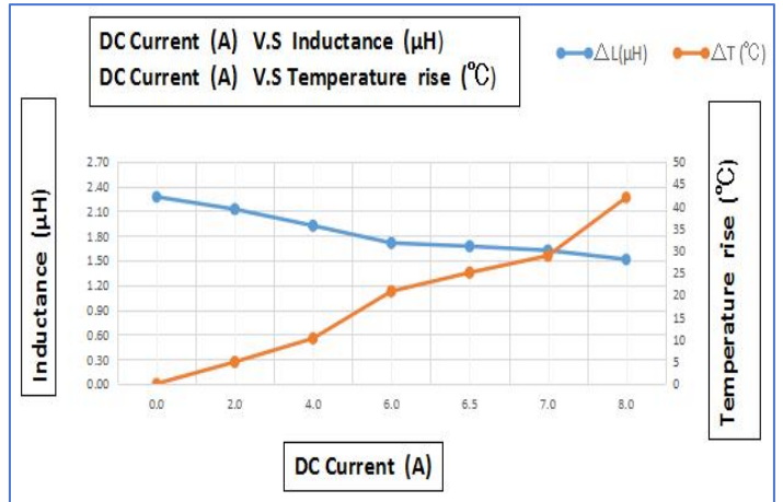
GSM0530-4R7-M
