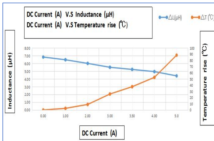
GSM0530-6R8-M
