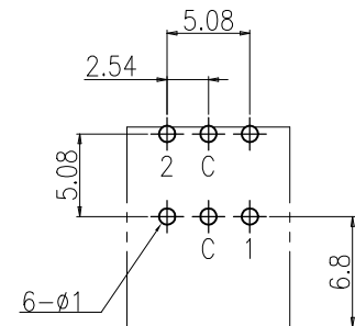
P.C.B DIMENSION (Top View)
